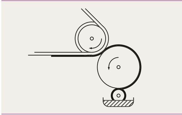
Diagram of a flexo-printing system suitable for applying AERODISP® as an anti-slip agent.
