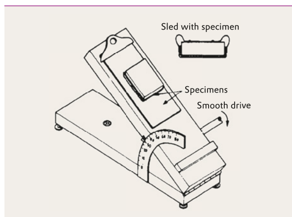
Static friction test device based on the TAPPI T-815 om-1 method.
