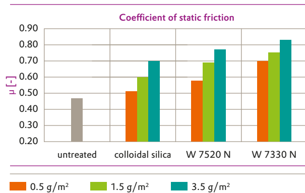
Comparison between the friction coefficients that can be achieved with colloidal silica, AERODISP® W 7520 N and AERODISP® W 7330 N with different weights of application.
