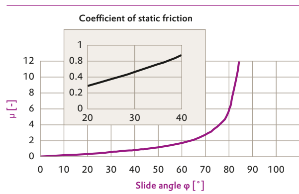
Correlation between the friction coefficient \mu and the slide angle \varphi for the entire angle range and for the angle range relevant for antislip applications.
