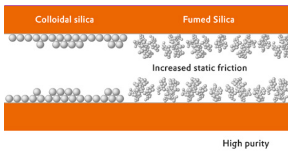
Model for increased static friction of a paper surface coated with AEROSIL® particles as opposed to conventional colloidal silica.
